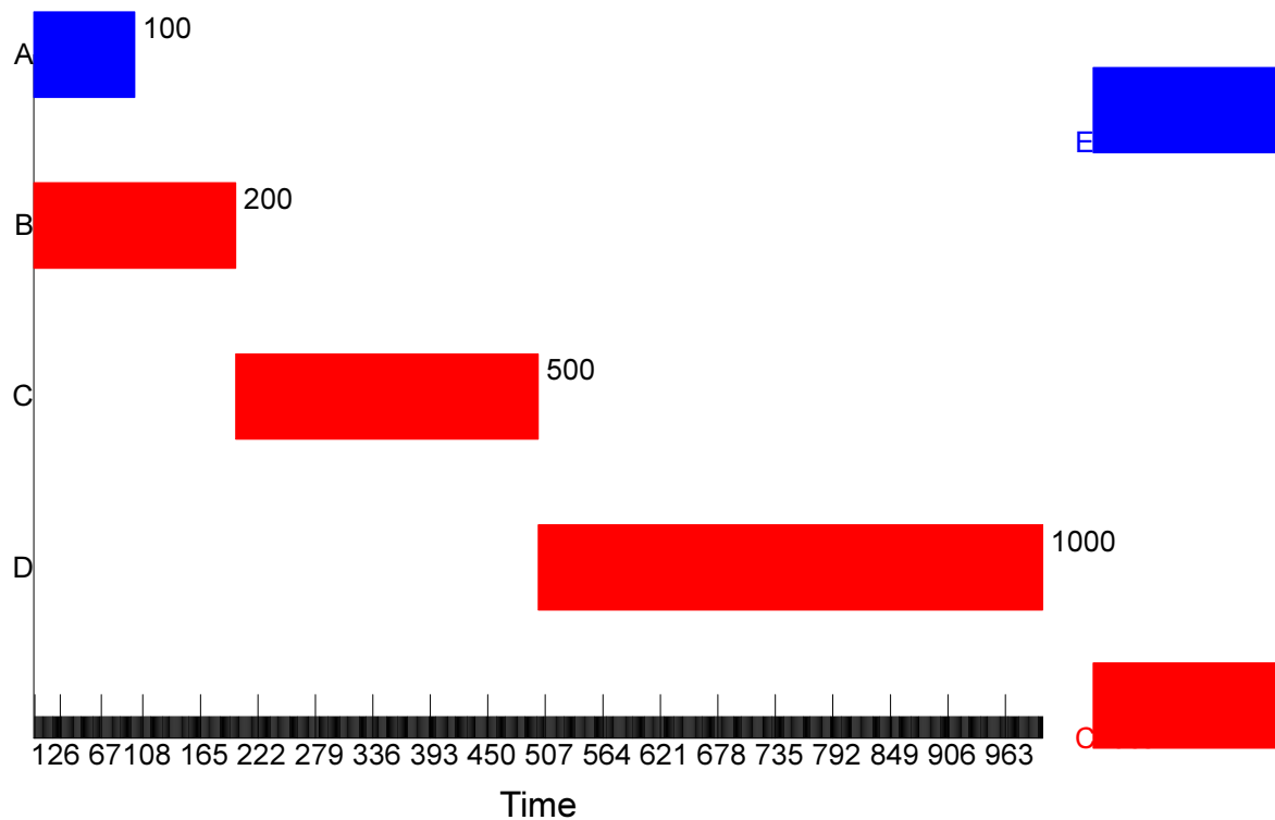
(untitled) Gantt chart (Early times)
