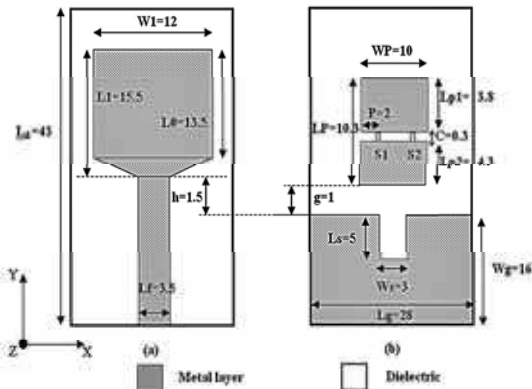
Fig. 1: Antenna geometry (a) Top View (b) Bottom View (unit: mm)
