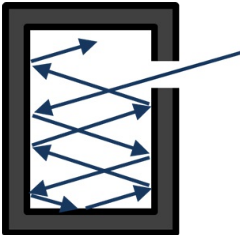
(Black body)
