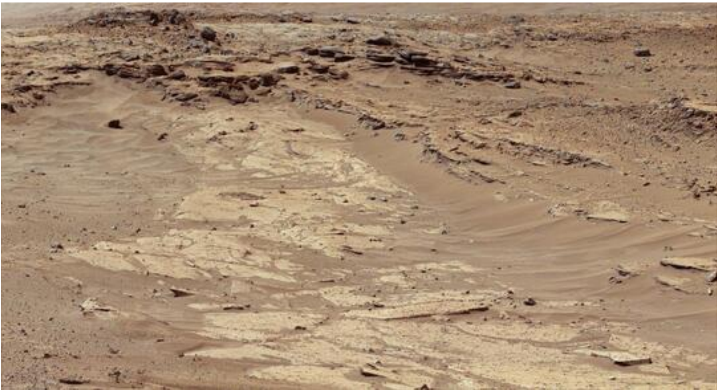
(Mars)
