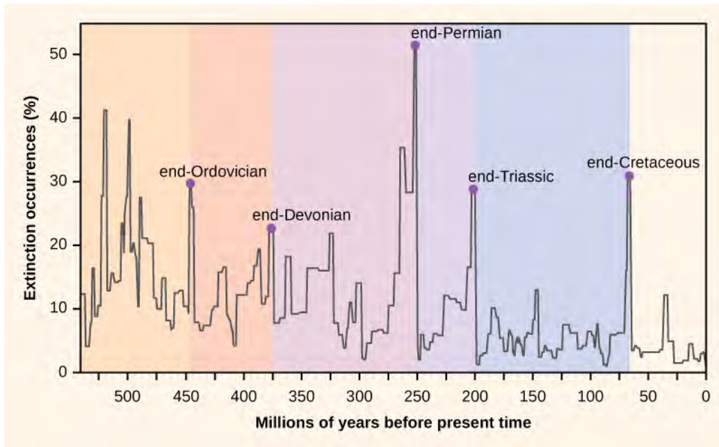
Figure 47.5 Percent extinction occurrences as reflected in the fossil record have fluctuated throughout Earth's history. Sudden and dramatic losses of biodiversity, called mass extinctions, have occurred five times.
