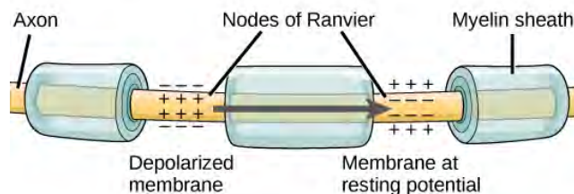
Figure 35.13 Nodes of Ranvier are gaps in myelin coverage along axons. Nodes contain voltage-gated K^+ and Na^+ channels. Action potentials travel down the axon by jumping from one node to the next.
