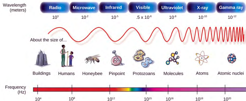
Figure 36.16 In the electromagnetic spectrum, visible light lies between 380 nm and 740 nm. (credit: modification of work by NASA)
