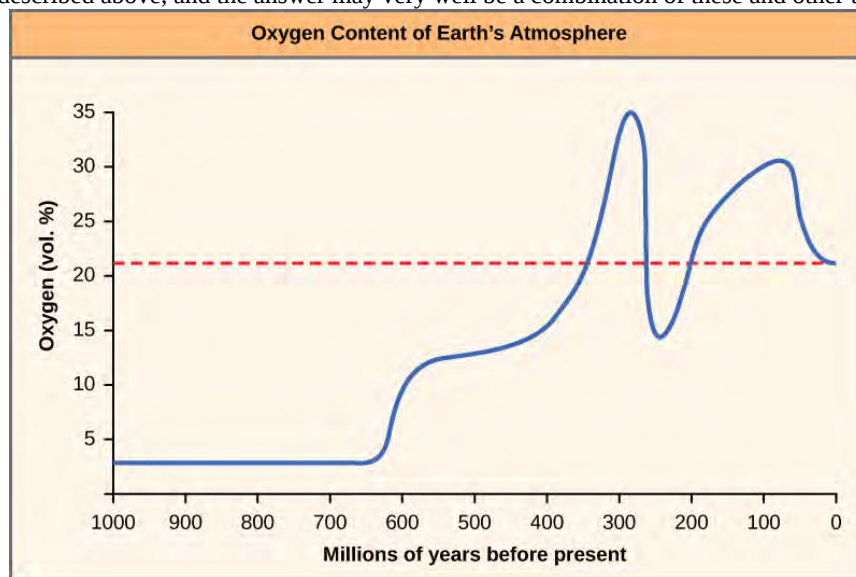
Figure 27.18 The oxygen concentration in Earth's atmosphere rose sharply around 300 million years ago.
